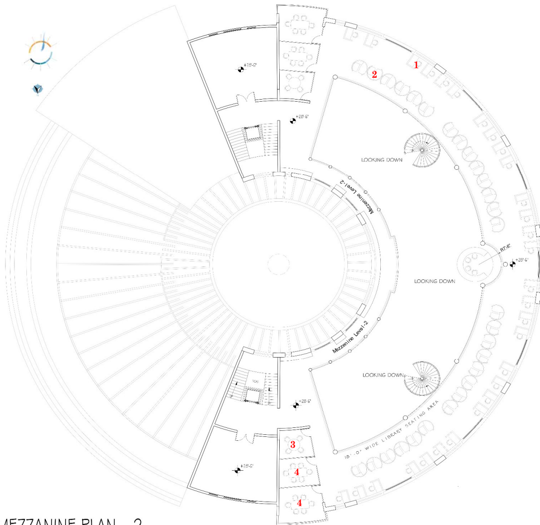
MEZZANINE PLAN - 2
